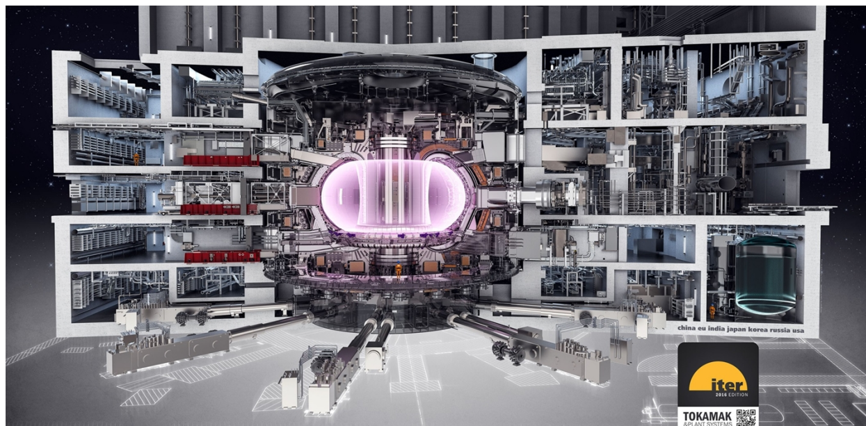
Figure 1. ITER Tokamak.
